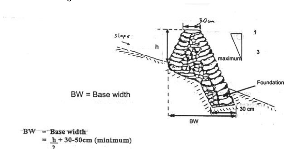
Figure 11: Technical standards of stone bund
