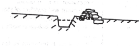
Figure 15: Integration of stone bunds with trenches
