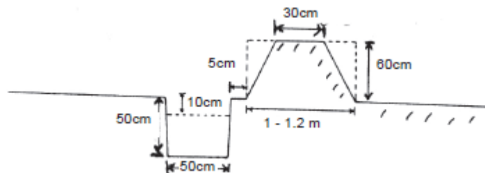
Figure 1: Technical drawing of soil bund for stable soil
