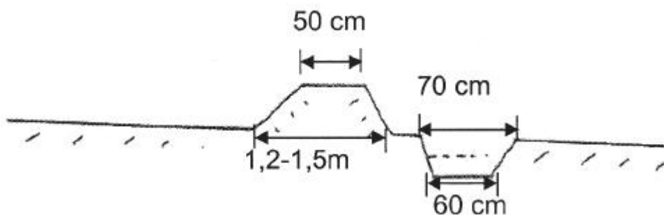
Figure 18: Fanya juu bund technical standard on unstable soil
