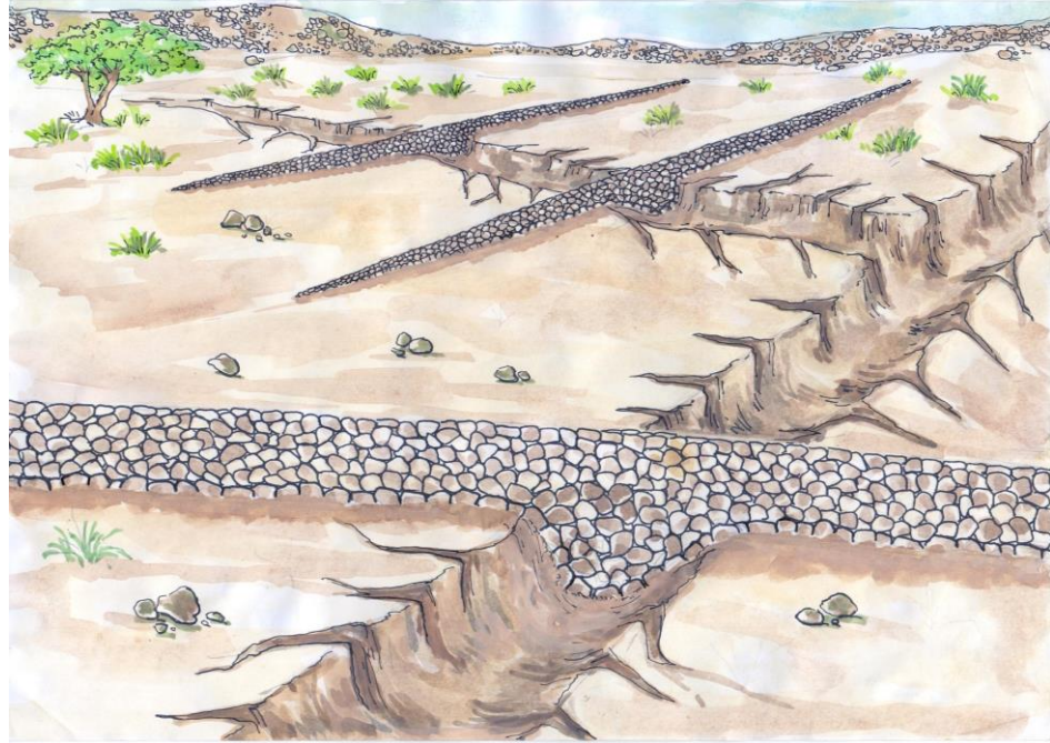
Illustration 4: Drystone structures can also be constructed within small gullies, but with a water spreading effect
