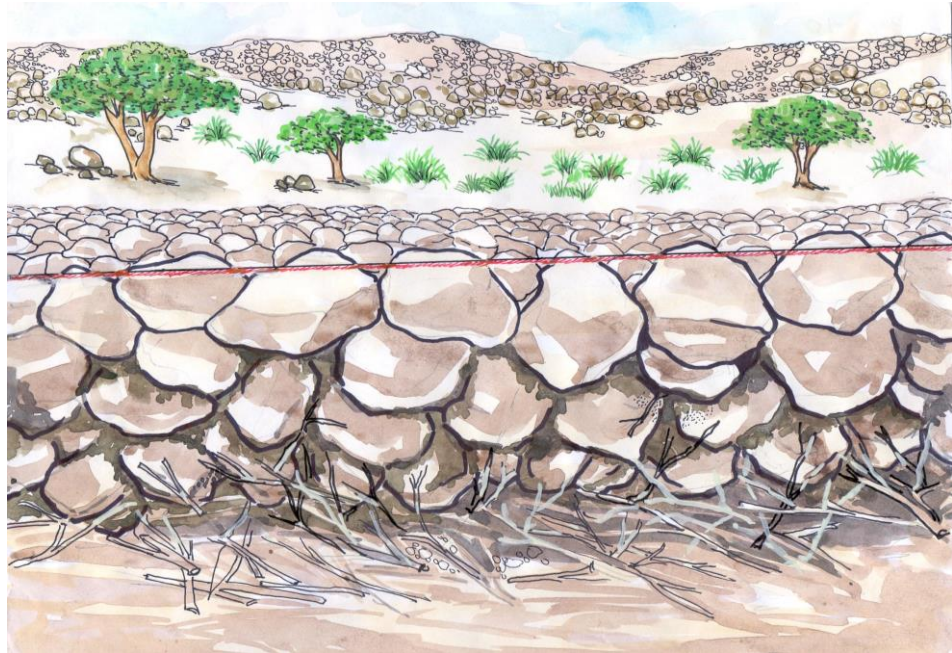
Illustration 18: The construction seen from upstream. The wall made of big stones, the rope demarcating the upper straight line of the dam. Small stones in the back indicate that the construction is not yet finished. A cover layer of big stones is missing.
